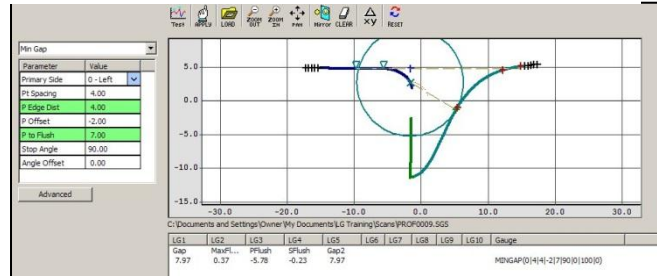
Scan Tested with Virtual Gauge in LGWorks
